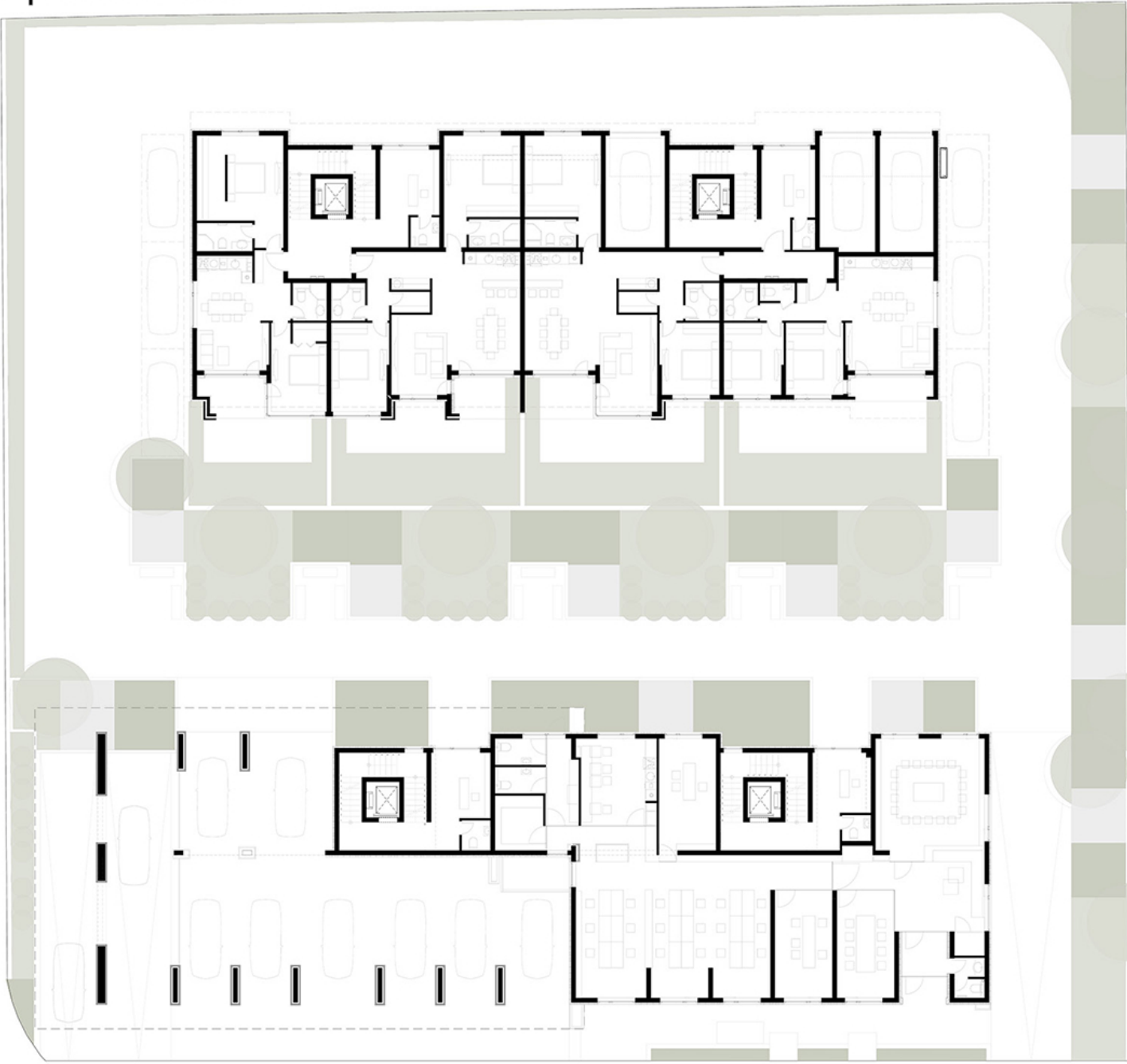
ПАРТЕР | GROUND LEVEL
