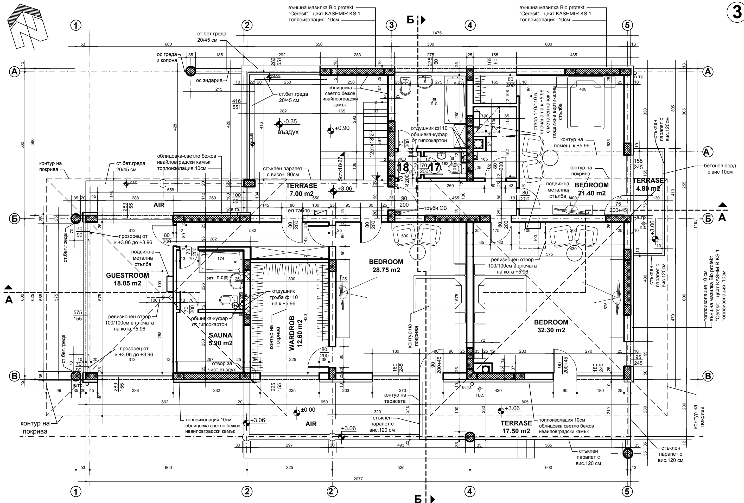
PLAN FN THE SECOND FLOOR M 1 : 75
